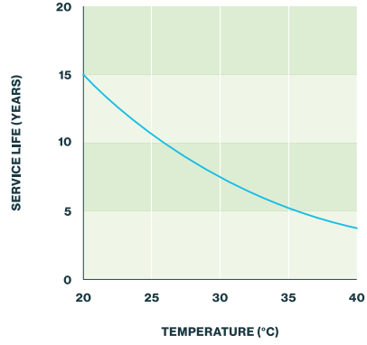
Service life vs. Temperature
